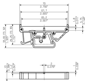
LOCKING-FOOT LEFT
