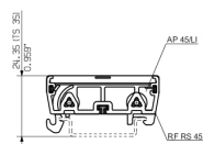
RAIL MOUNTING
