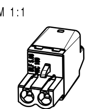
BLF 5.08/02/180 (Standard)
