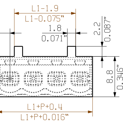
MIN. FRONT PLATE CUT-OUT
