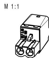
BLF 5.08/02/180 (Standard)
