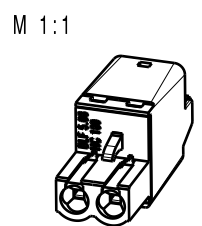
BLF 5.08/02/180 (Standard)
