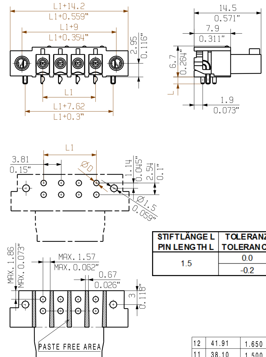
BCL-SMT 3.81/.../90LF 1.5...
