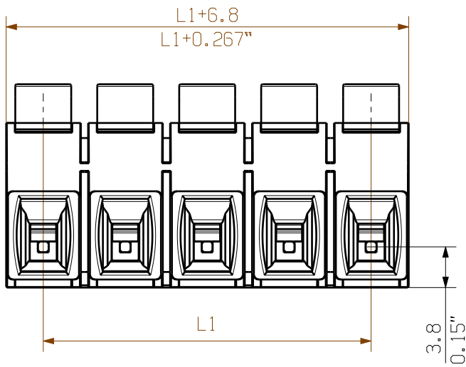
SLZ7.62HP/.../180G
