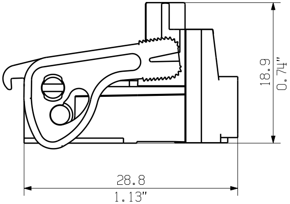
SLZ7.62HP/.../180G
