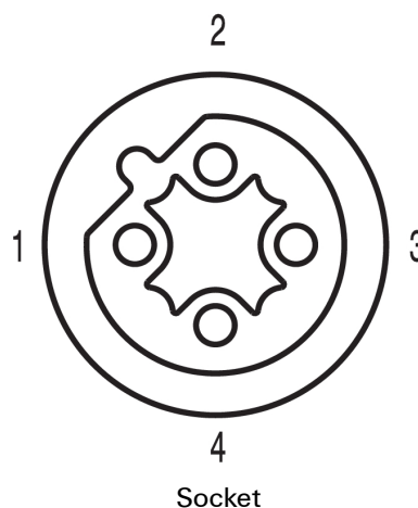
Straight socket
