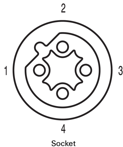
Straight socket
