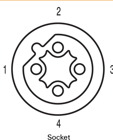
Angled socket
