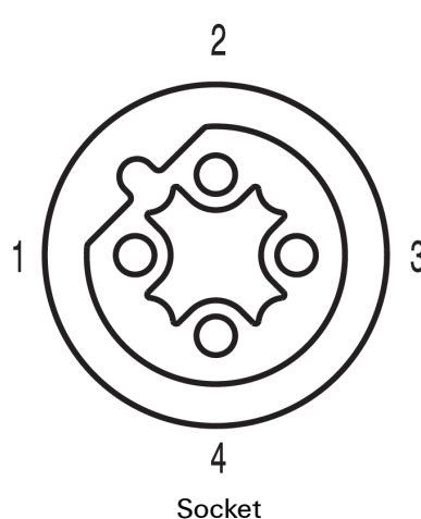
Angled socket
