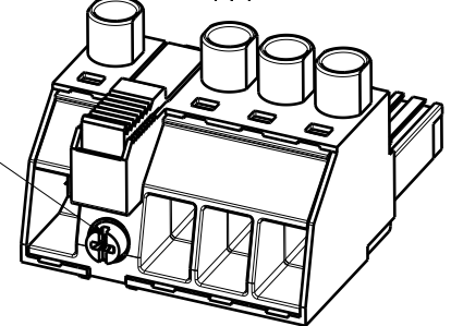
BVZ 7.62IT/04/180M(S)F4 1:1
