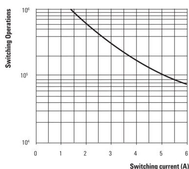
Electrical endurance 230 V AC resistive load
