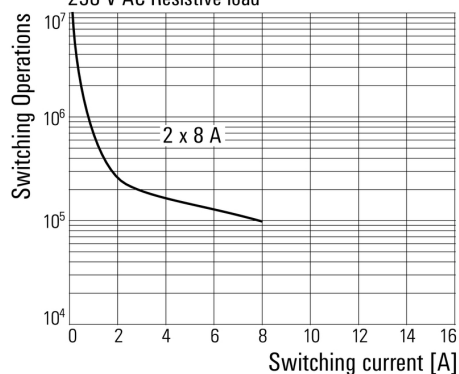
Electrical endurance
