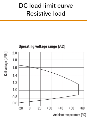
AC operational voltage range
