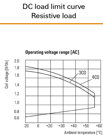
AC operational voltage range
