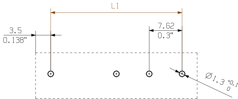
HOLE PATTERN
