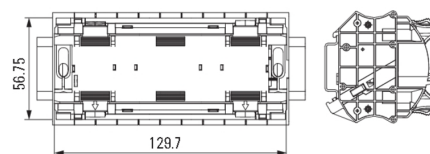
Mounting rail
