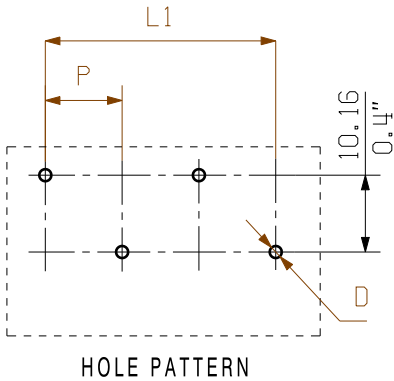
HOLE PATTERN
