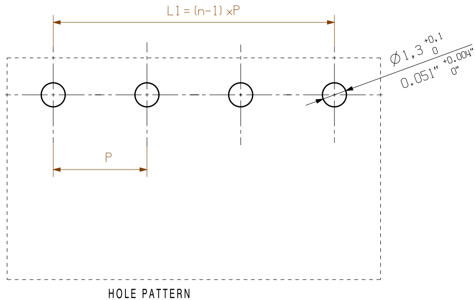
HOLE PATTERN
