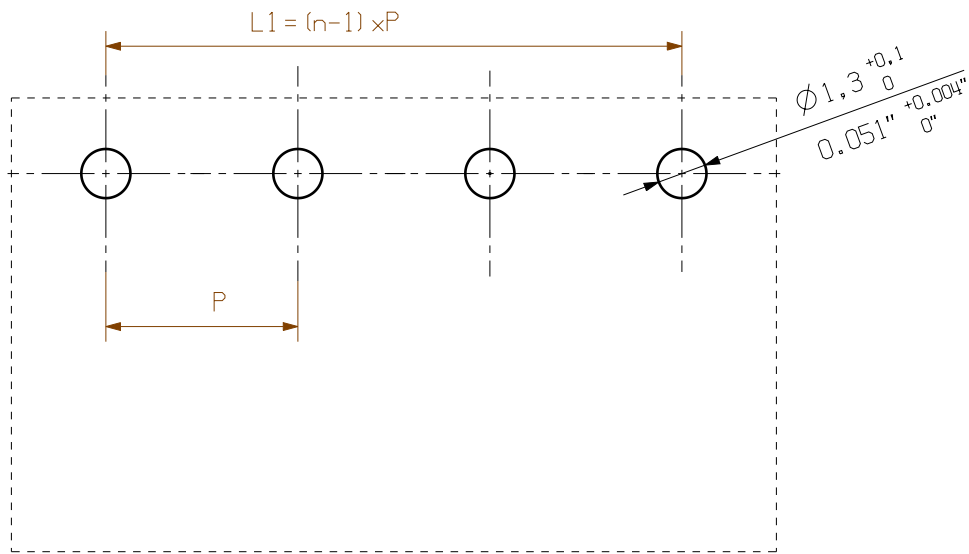
HOLE PATTERN
