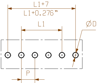
hole pattern
