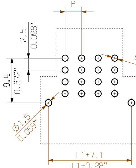
HOLE PATTERN
