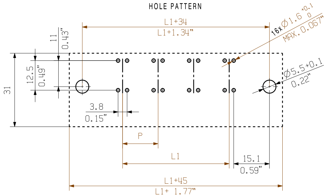
HOLE PATTERN
