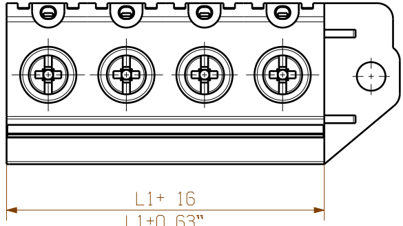
HOLE PATTERN
