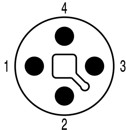
Pole scheme
