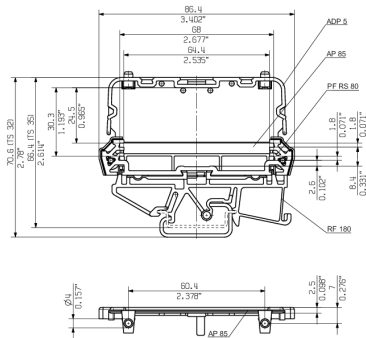
RAIL MOUNTING FOR BOTH SIDES (RIGHT AND LEFT)
