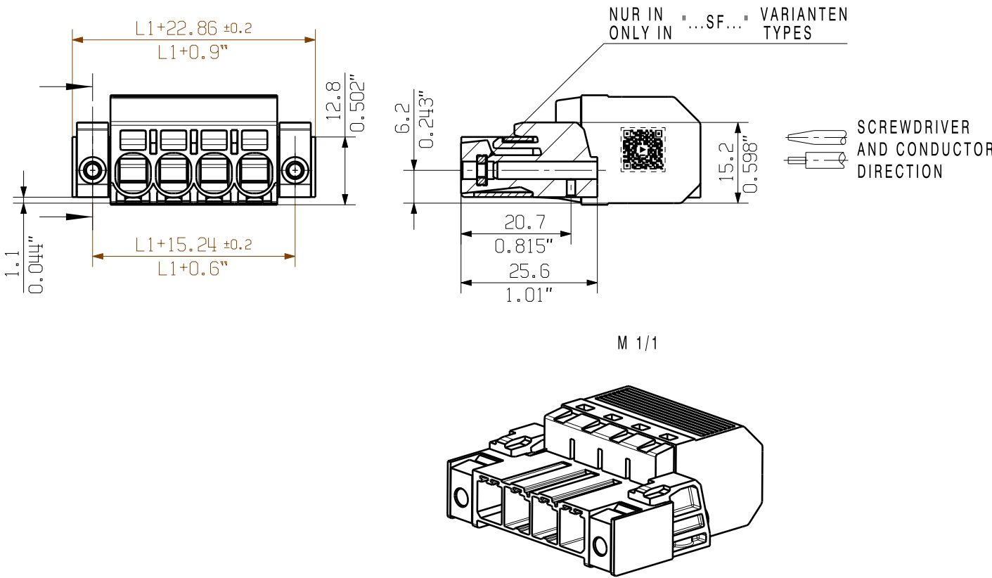
SHOWN: SVF7.62HP/04/180SF
