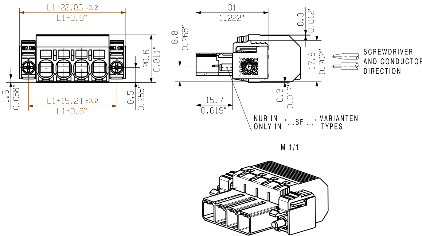
SHOWN: SVF7.62HP/04/180SFI
