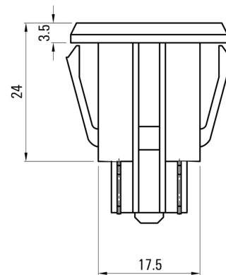
Dimensioned drawing
