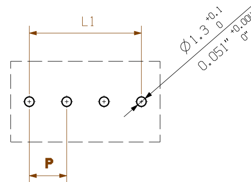
HOLE PATTERN
