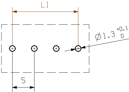
HOLE PATTERN
