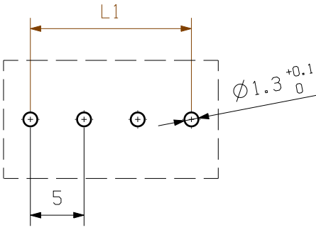
HOLE PATTERN
