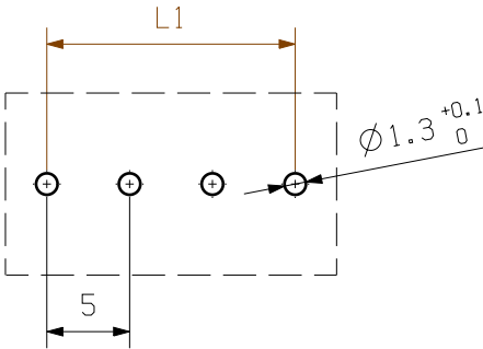
HOLE PATTERN
