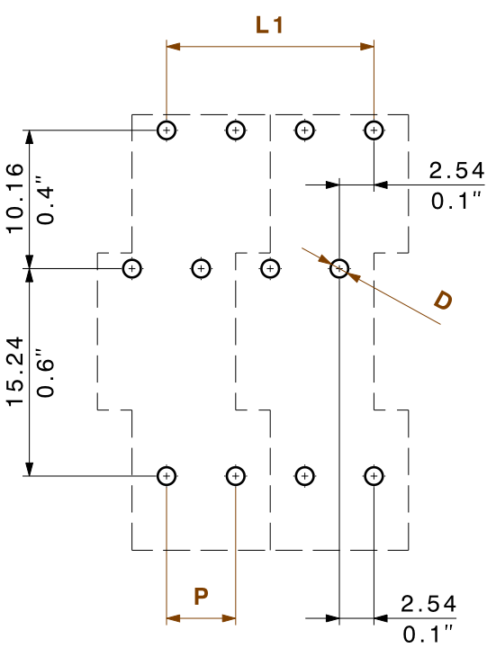
HOLE PATTERN
