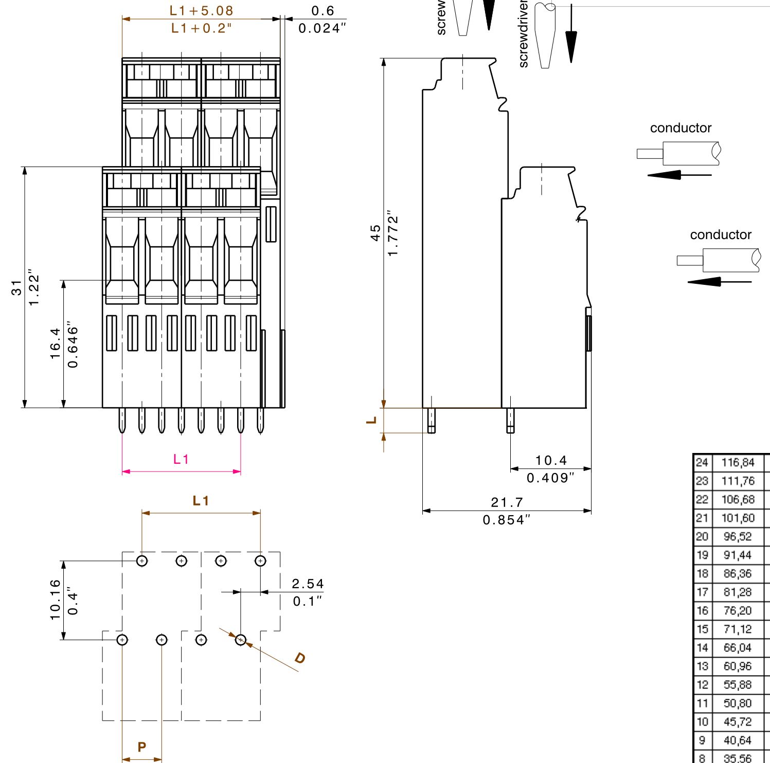
Layout finished holes
