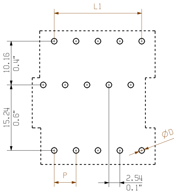
PCB LAYOUT
