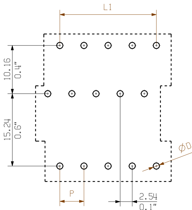
PCB LAYOUT
