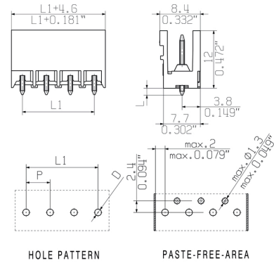
HOLE PATTERN
