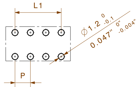
HOLE PATTERN
