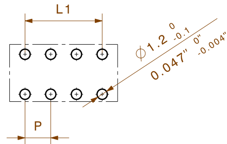
HOLE PATTERN
