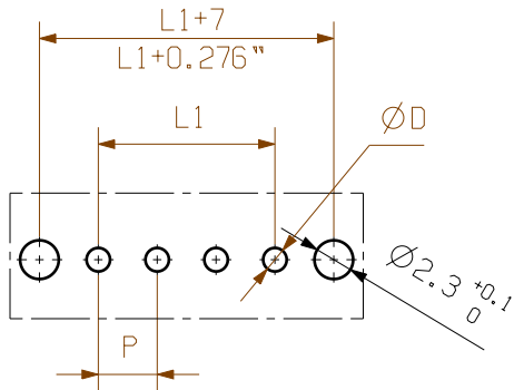
hole pattern
