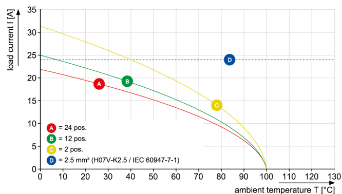
BLT 5.08HC/18/180 - SL-SMT 5.08HC/18/90
