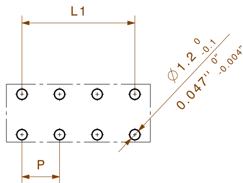
HOLE PATTERN
