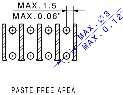
PASTE-FREE AREA
