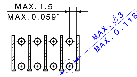
PASTE-FREE AREA
