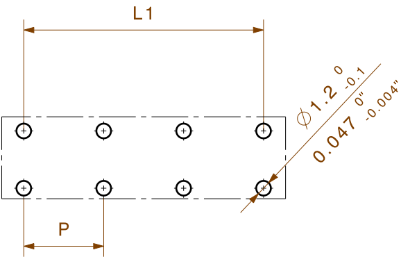
HOLE PATTERN
