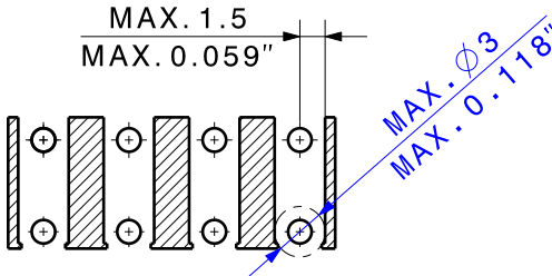
PASTE-FREE AREA
