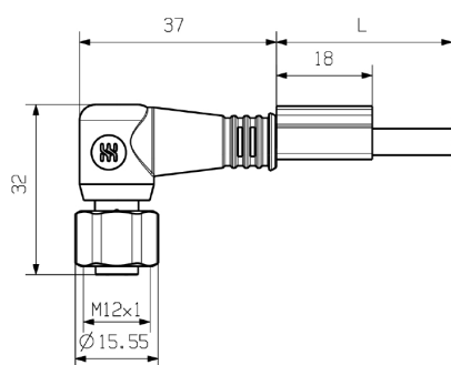
Angled socket
