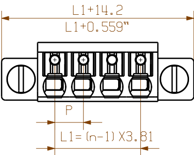
BCF 3.81/.../180F ...
